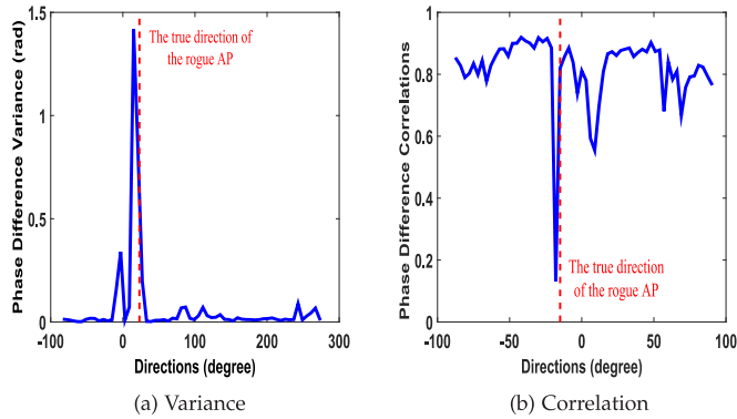
Fig. 7. Illustration of applying the phase difference methods when the user moves around the laptop with 1 feet distance: (a) variance of phase difference and (b) correlation coefficient of phase difference.
