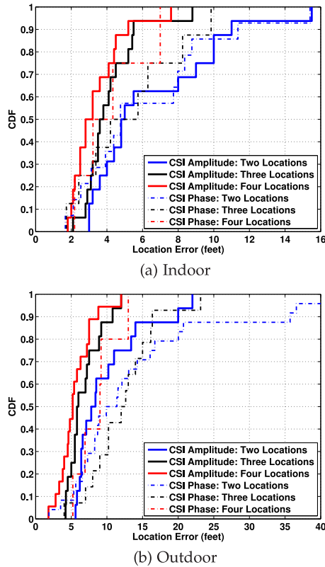
Fig. 13. Position estimation performance via geometric relationship based method while using CSI amplitude and phase for direction derivation, respectively.
