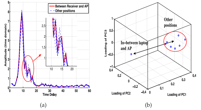
Fig. 6. Illustration of using amplitude orthogonal transformation method: (a) Time domain CSI amplitude at eight different positions around the wireless device: the correlation between the positions is over 94 percent. (b) After using amplitude orthogonal transformation method while three principal components are considered.
