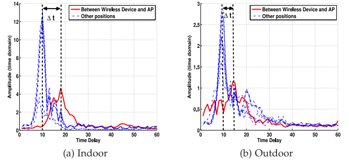
Fig. 3. CSI amplitude in time domain at eight different positions around the wireless device: time delay phenomenon in simple wireless environments.
