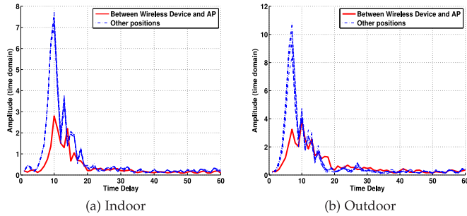
Fig. 4. CSI amplitude in time domain at eight different positions around the wireless device: time delay phenomenon in complex wireless environments.
