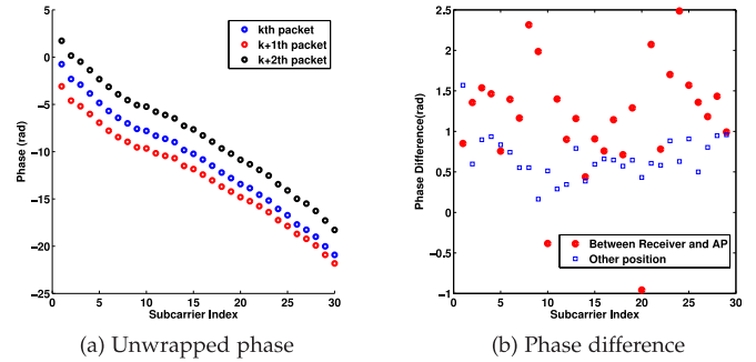
Fig. 5. Illustration of CSI phase in the frequency domain: (a) unwrapped phase from three consecutive packets and (b) phase difference when user stands at different positions.
