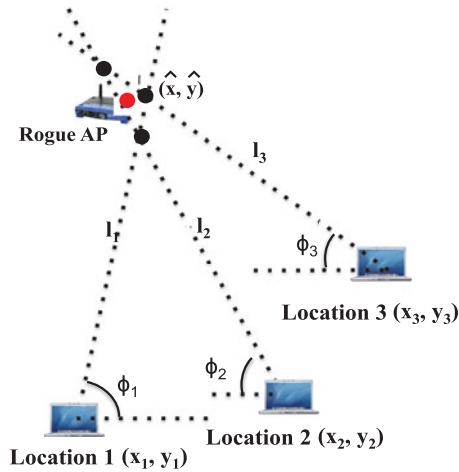
Fig. 8. Illustration of position estimation of the rogue AP through geometric relationship based method while conducting direction determination at three different locations.
